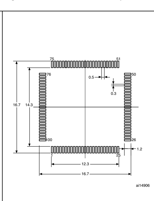
Figure 69. Recommended footprint (1)(2)
